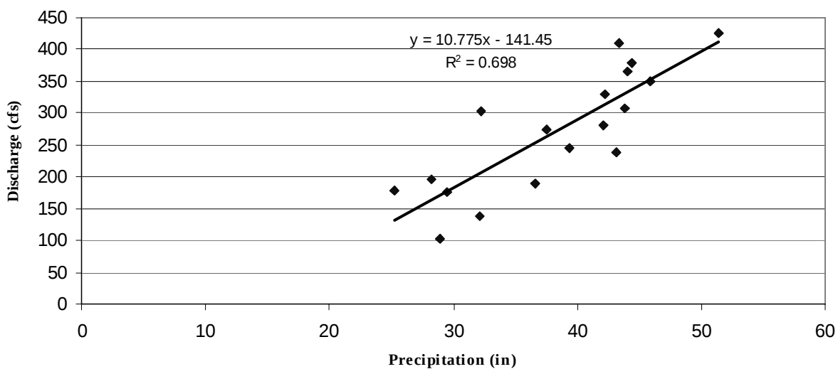
Figure 6. Mean Annual Precipitation vs. Annual Discharge for Beacon, NY - 1950-1967
